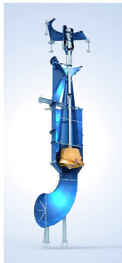
ANDRITZ vertical line shaft pump
